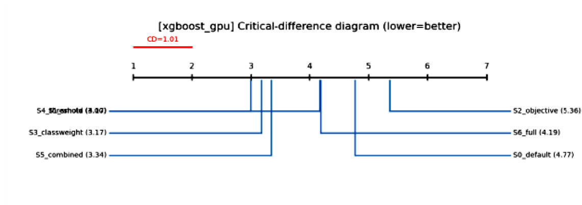
Fig 4.6: Critical-Difference Diagram (XGBoost-GPU)
