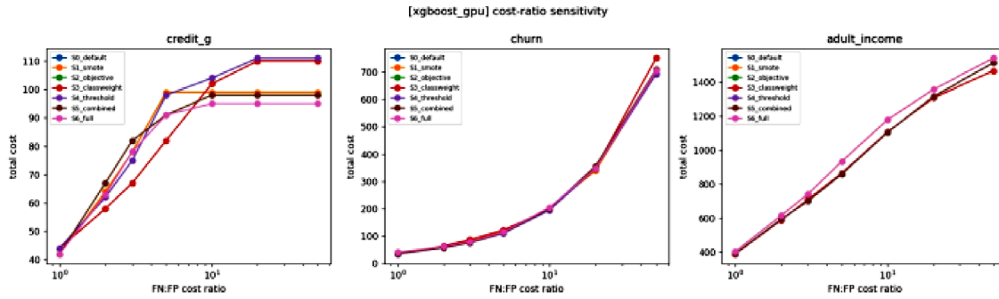
Fig 4.17: Cost-Ratio Sensitivity (XGBoost-GPU)
