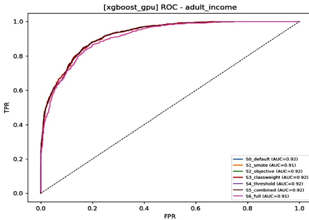
Fig 5.7: ROC Curves – Adult Income
