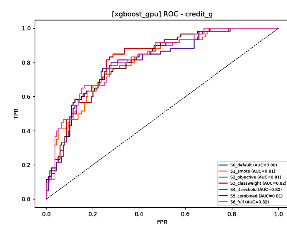
Fig 5.5: ROC Curves – Credit G (Secondary Ranking View)
