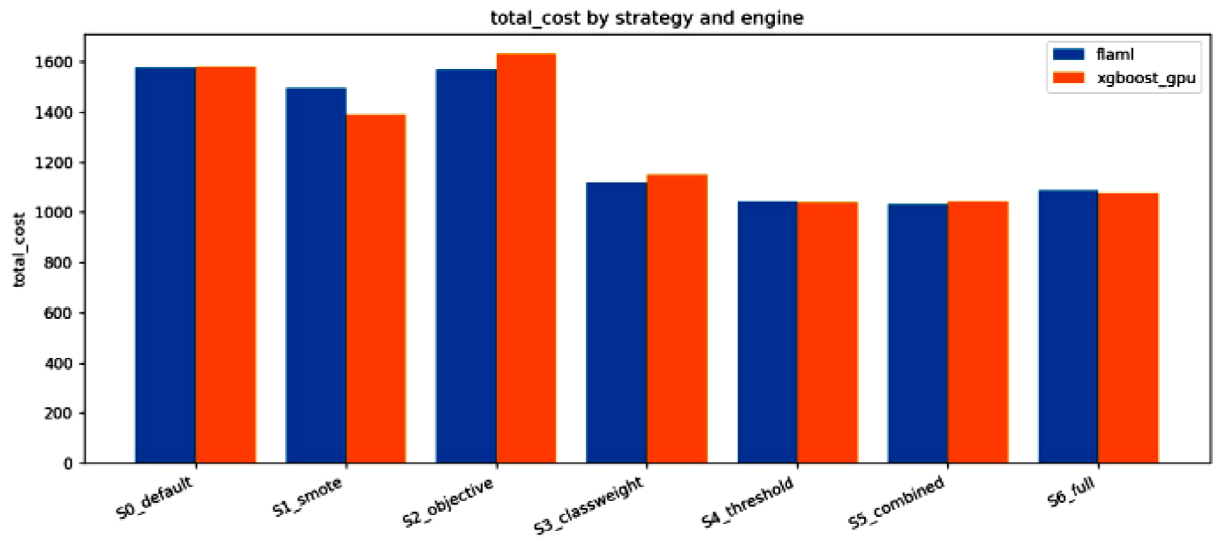
Fig 4.13: Total Cost by Strategy and Engine
