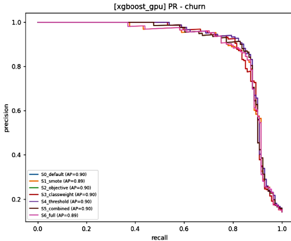
Fig 5.3: Precision-Recall Curves – Churn (14% Minority)
