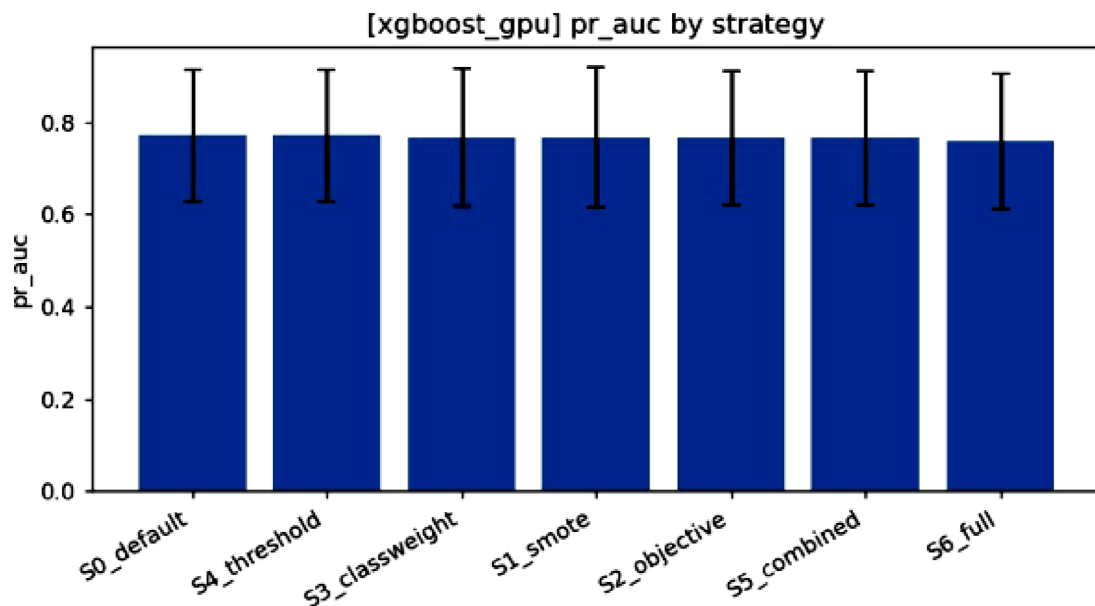
Fig 4.3: Mean PR-AUC by Strategy (XGBoost-GPU)
