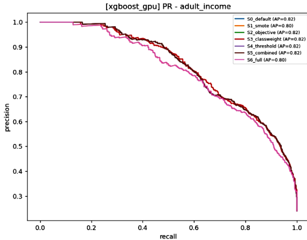
Fig 5.4: Precision-Recall Curves – Adult Income (24% Minority)
