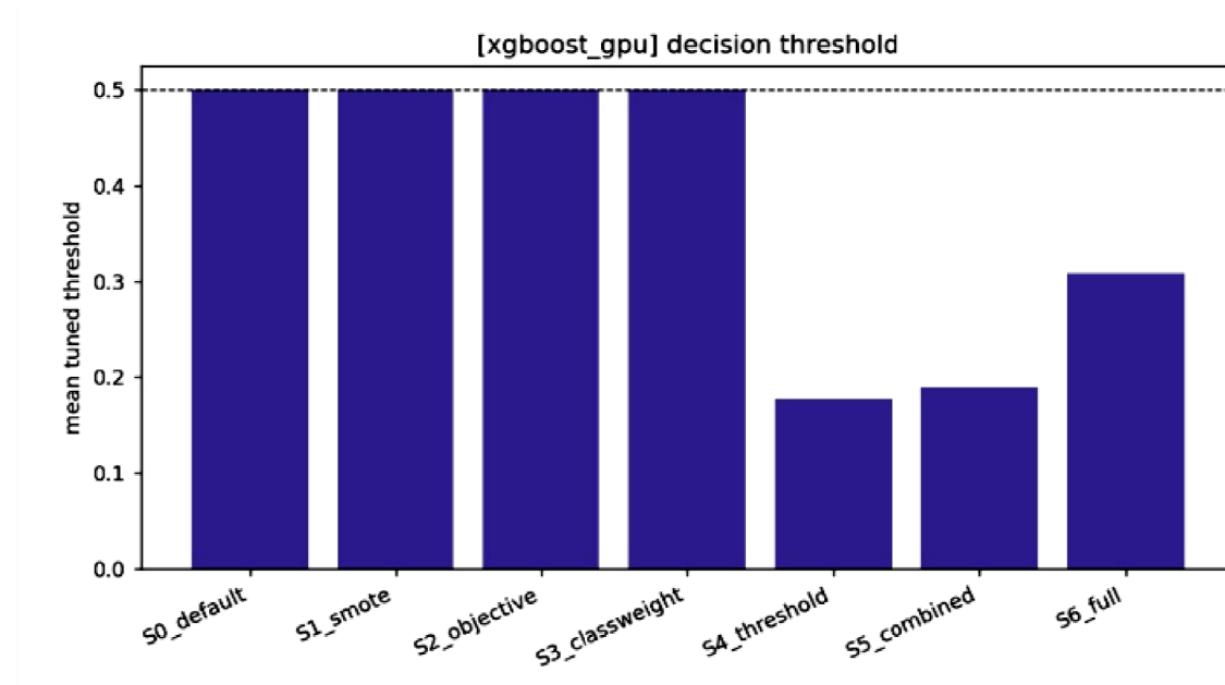
Fig.5.1: Mean Tuned Threshold by Strategy (XGBoost-GPU)
