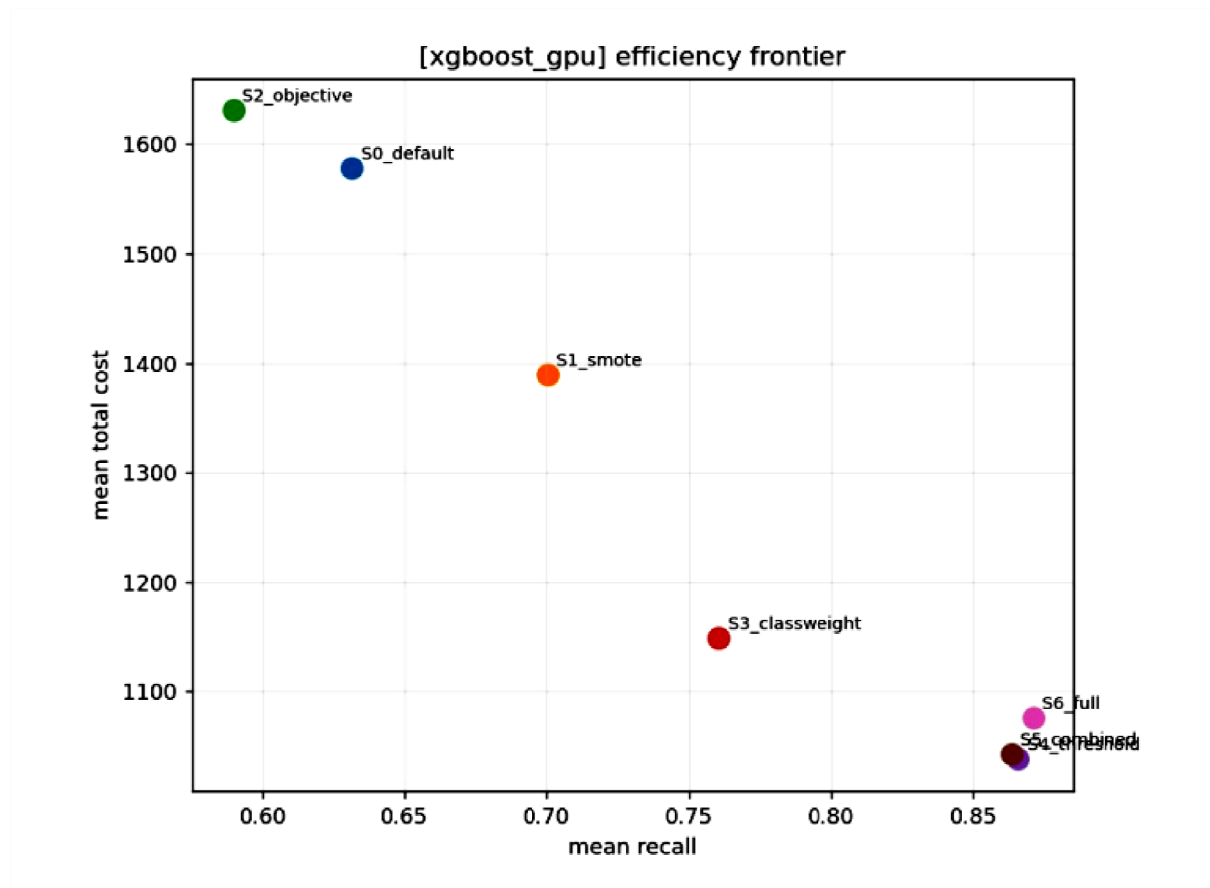
Fig 5.8: Efficiency Frontier – Recall vs Total Cost (One-Figure Summary)
