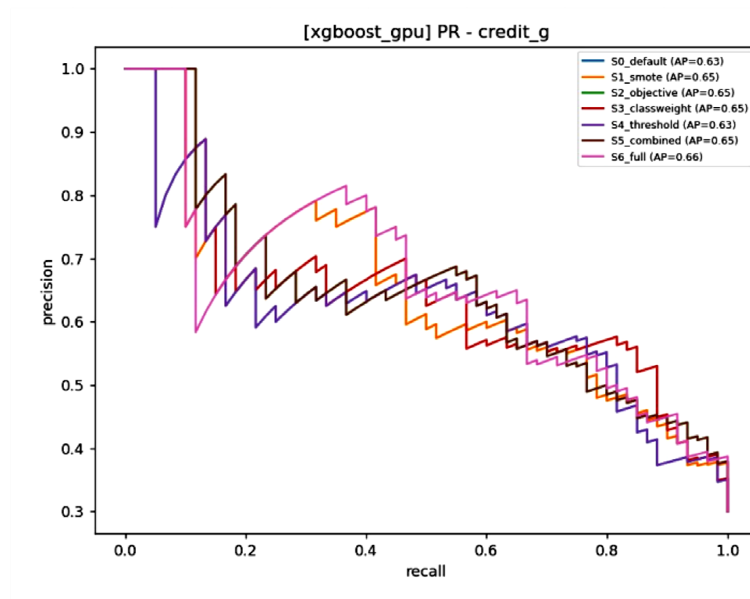
Fig 5.2: Precision-Recall Curves – Credit G (30% Minority)
