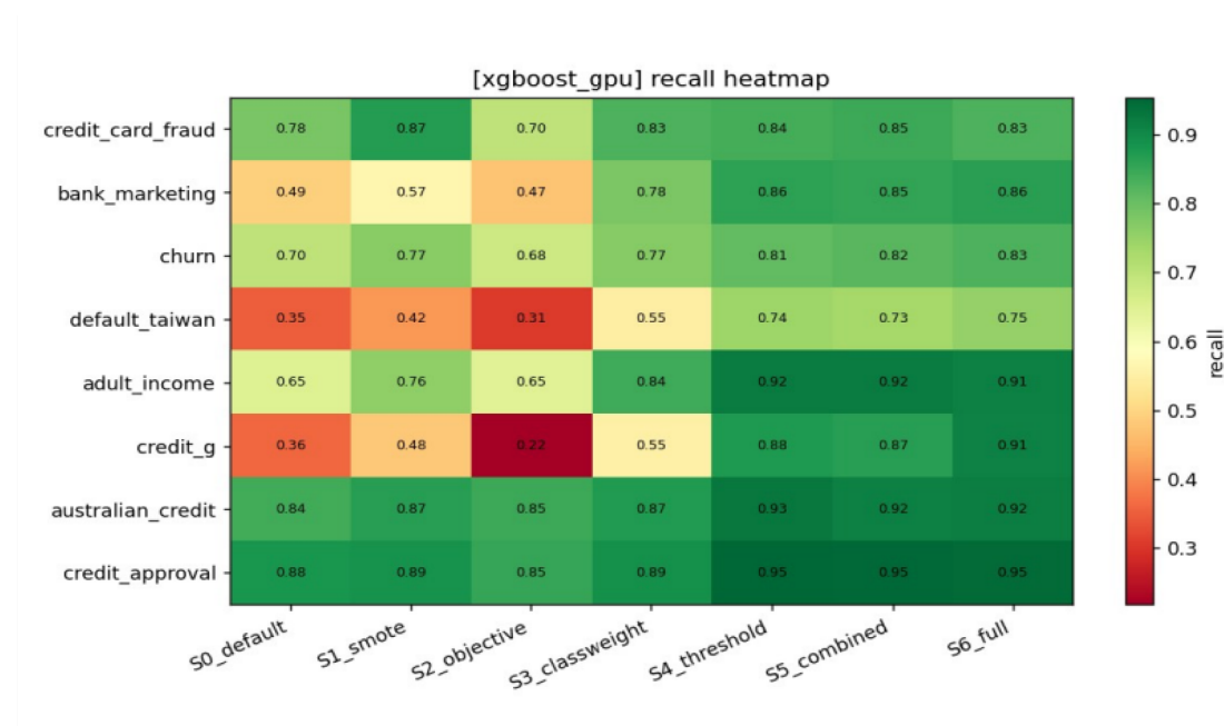
Fig 4.11: Recall Heatmap (XGBoost-GPU)
