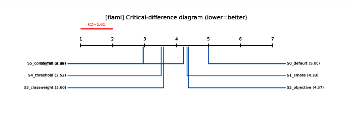
Fig 4.7: Critical-Difference Diagram (FLAML)
