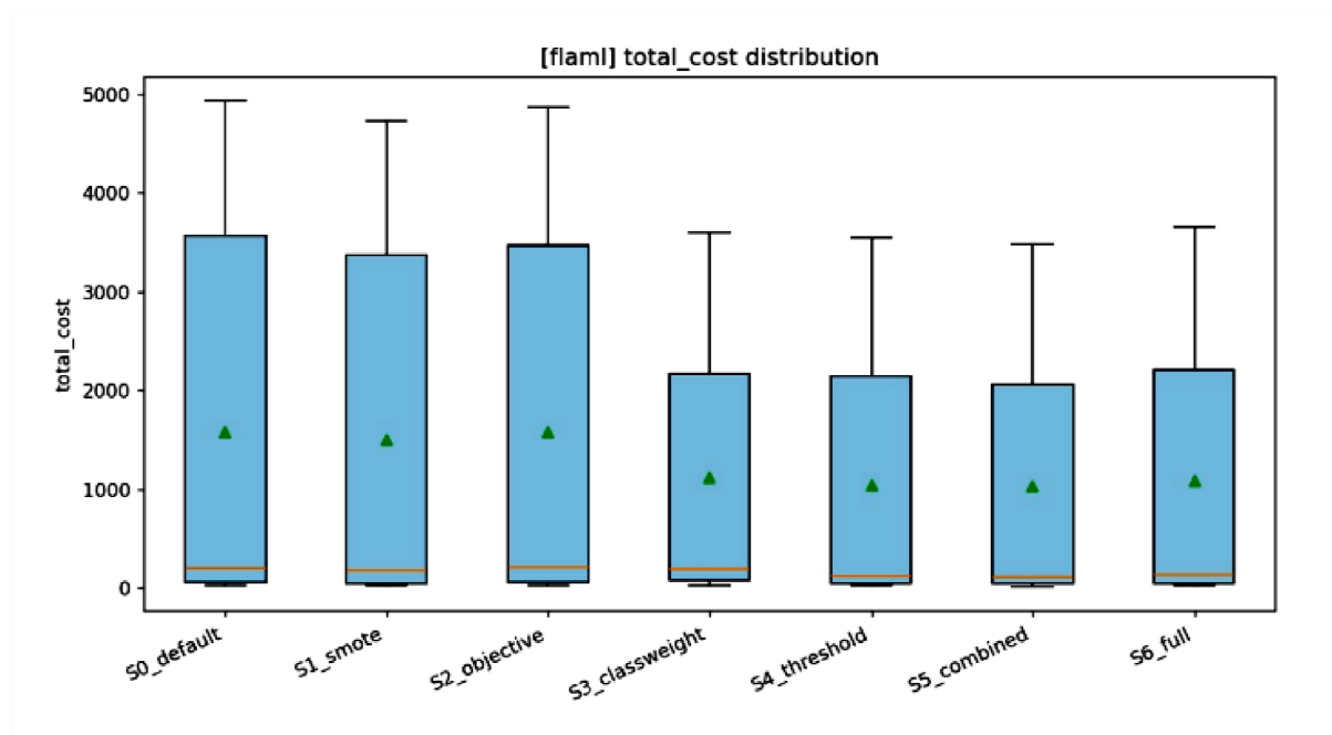
Fig A.1: Total Cost Distribution by Strategy (FLAML)
